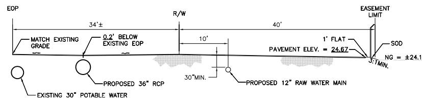
SECTION (Y-Y)
