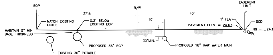
SECTION (Y-Y)
